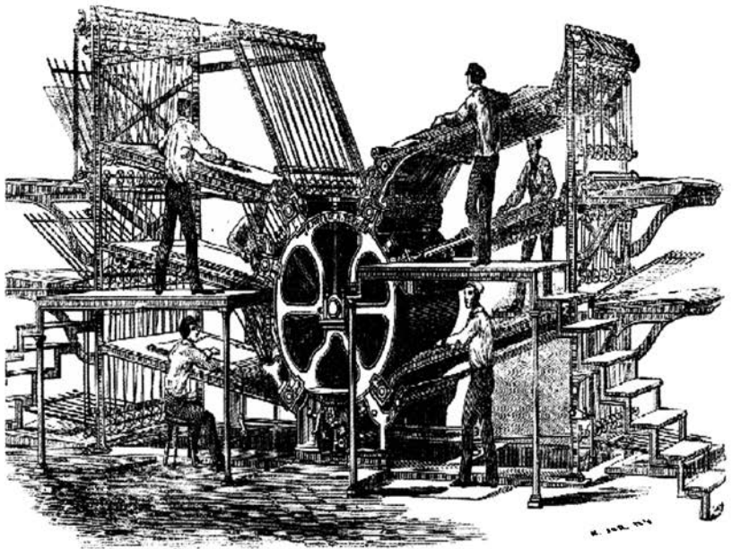
FIG. 6. SIX-CYLINDER PRINTING PRESS.
