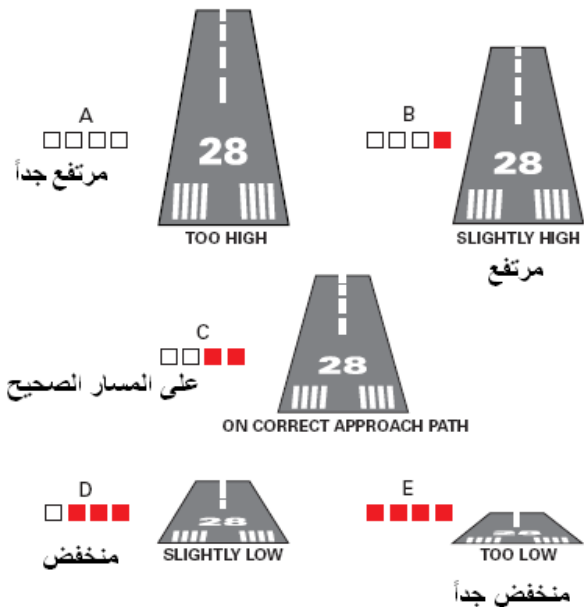
Typical PAPI System
